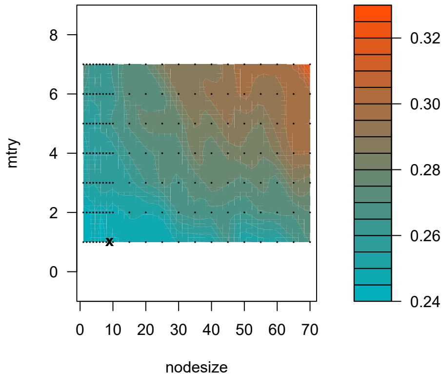
RandomForest OOB error for nodesize & mtry
